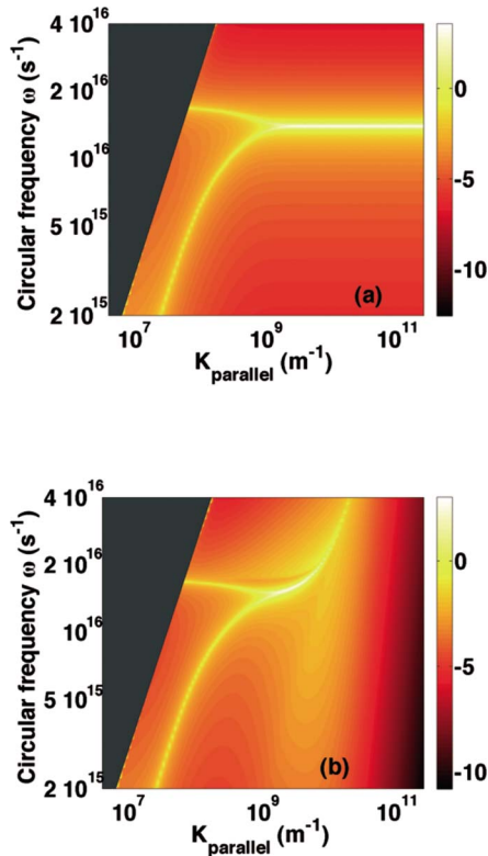
FIG. 6. (Color online) Plot of the expression \text{Im}(r_p^{31})^2 / [1 - r_p^2 e^{-2\gamma_3'' d}]^2 that appears in the integrand [Eq. (3)] of the heat flux for evanescent waves ( K > \omega/c ). The gap size is 2 nm here. The color bar is in logarithmic scale. (a) Local model. (b) Nonlocal Boltzmann-Mermin model. A Lindhard-Mermin model would cut more strongly the integrand at large parallel wave vectors.
